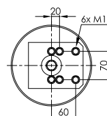
PLASTIC PISTON
