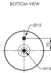
STEEL PISTON
