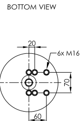
STEEL PISTON
