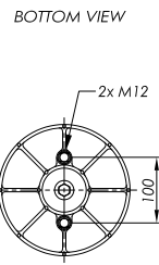
PLASTIC PISTON
