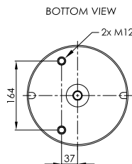
STEEL PISTON
