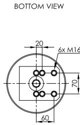
PLASTIC PISTON
