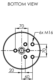
STEEL PISTON
