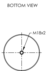
STEEL PISTON
