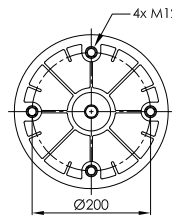
PLASTIC PISTON
