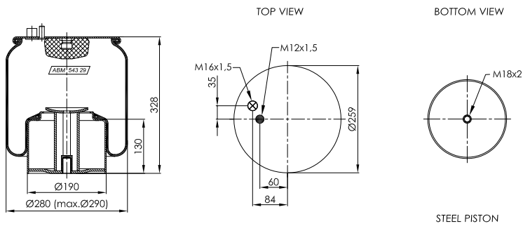
STEEL PISTON
