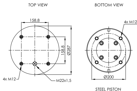
STEEL PISTON
