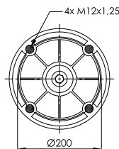
PLASTIC PISTON
