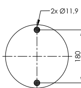
STEEL PISTON
