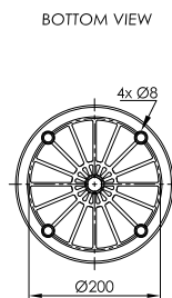
PLASTIC PISTON
