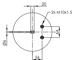
STEEL PISTON
