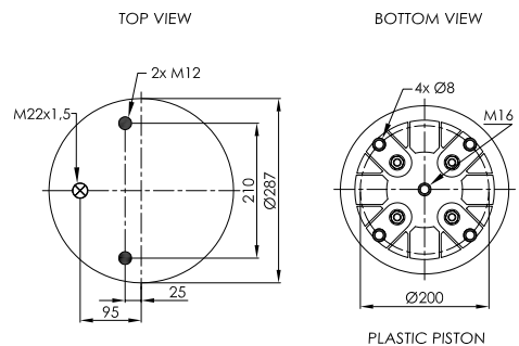
PLASTIC PISTON
