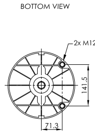
PLASTIC PISTON
