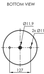
STEEL PISTON
