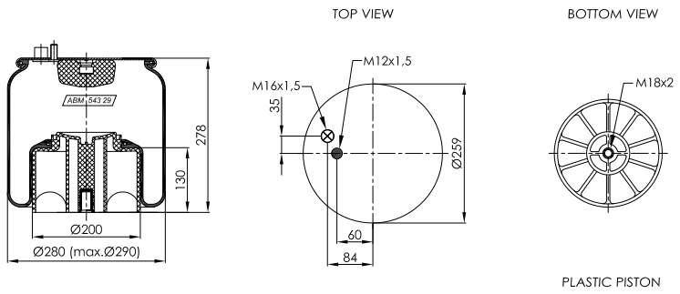
PLASTIC PISTON
