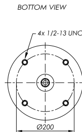
STEEL PISTON
