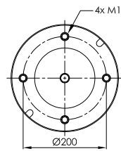
STEEL PISTON
