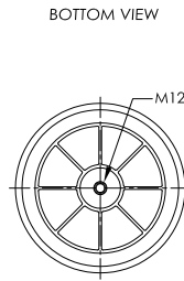
PLASTIC PISTON
