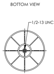
PLASTIC PISTON
