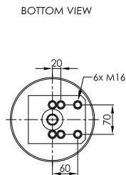
PLASTIC PISTON
