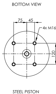
STEEL PISTON
