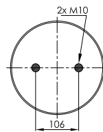
STEEL PISTON
