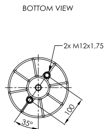
PLASTIC PISTON
