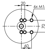
STEEL PISTON
