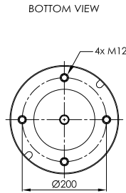
STEEL PISTON
