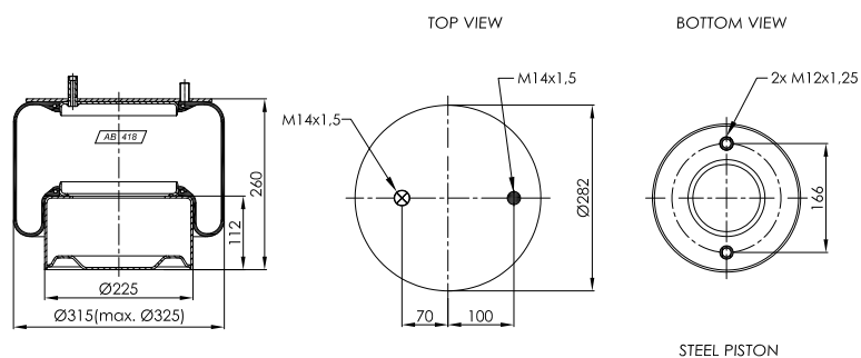
STEEL PISTON
