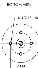
STEEL PISTON
