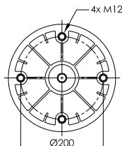
PLASTIC PISTON
