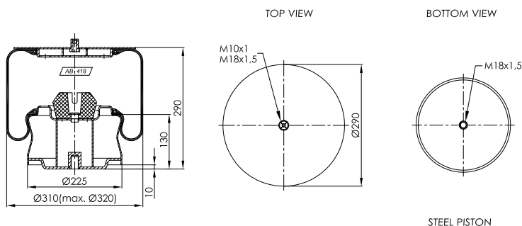
STEEL PISTON
