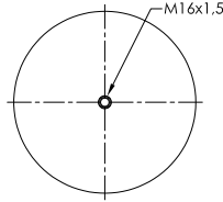
STEEL PISTON
