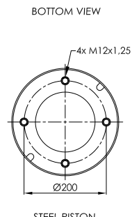
STEEL PISTON
