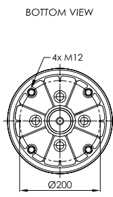
PLASTIC PISTON
