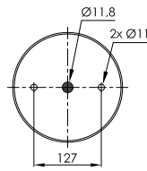
STEEL PISTON
