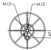
PLASTIC PISTON
