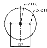
STEEL PISTON
