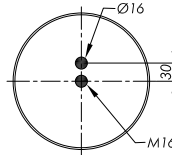
STEEL PISTON
