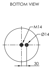
STEEL PISTON
