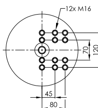
STEEL PISTON
