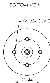
STEEL PISTON
