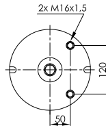
STEEL PISTON
