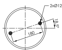
STEEL PISTON
