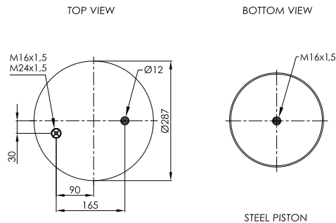
STEEL PISTON
