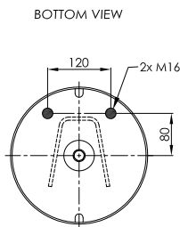
STEEL PISTON
