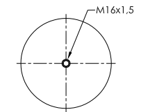
STEEL PISTON
