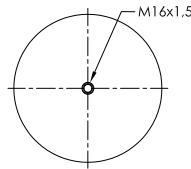
STEEL PISTON
