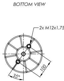
PLASTIC PISTON
