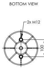
PLASTIC PISTON
