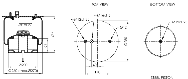
STEEL PISTON
