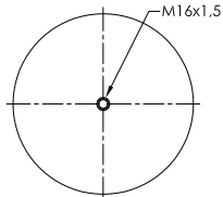
STEEL PISTON
