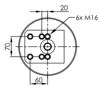
PLASTIC PISTON
