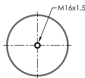
STEEL PISTON
