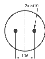
STEEL PISTON
