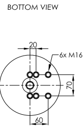
STEEL PISTON
