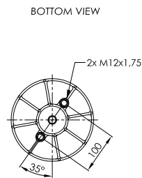
PLASTIC PISTON
