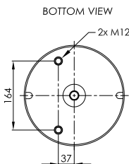
STEEL PISTON
