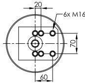
PLASTIC PISTON
