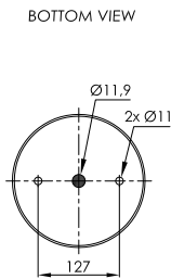
STEEL PISTON
