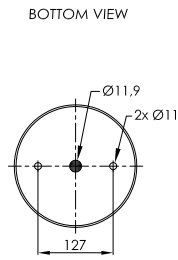
STEEL PISTON
