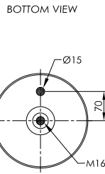
STEEL PISTON
