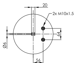
STEEL PISTON
