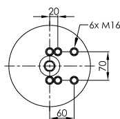
STEEL PISTON
