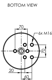
STEEL PISTON
