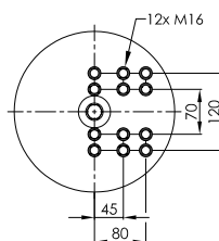
STEEL PISTON
