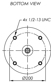
STEEL PISTON
