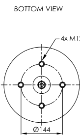
STEEL PISTON
