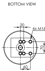
PLASTIC PISTON
