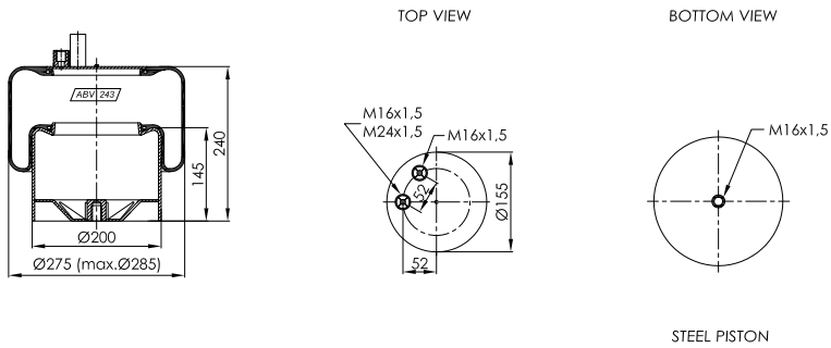
STEEL PISTON
